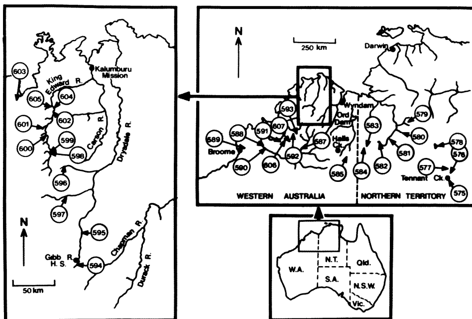
FIG. 1 Position of sample localities
